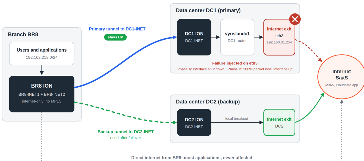
Figure 2. Lab topology: primary tunnel to DC1, backup tunnel to DC2, failure injected on DC1's internet exit (vyoslandc1, eth3).
