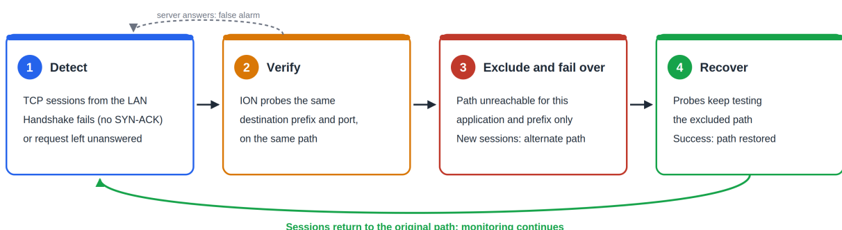
Figure 1. The Application Unreachability Detection cycle: detect, verify, exclude and fail over, recover.
